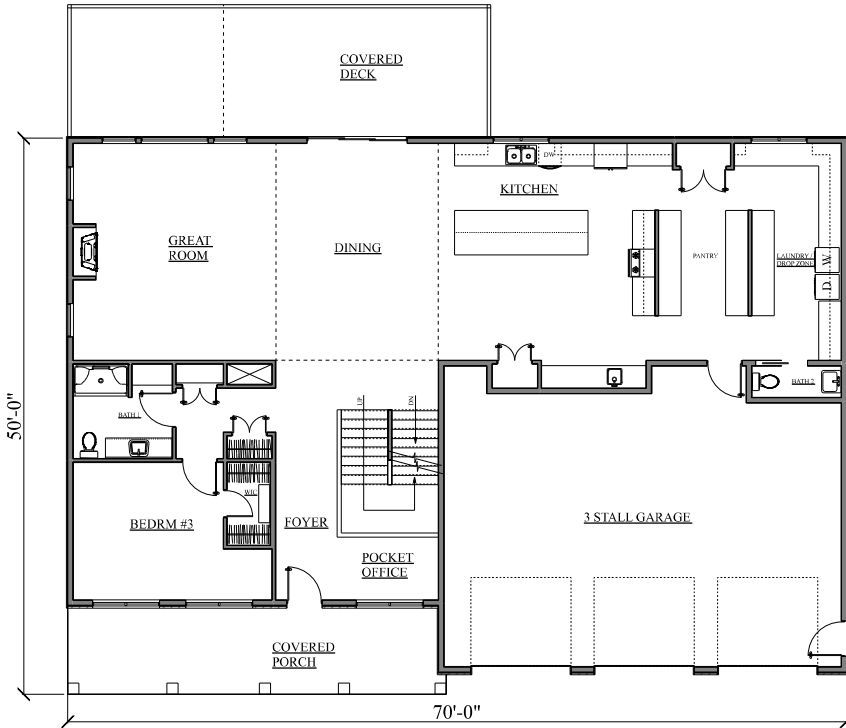
COPYRIGHT / 2020 / MIKE PRULL MAIN FLOOR PLAN
