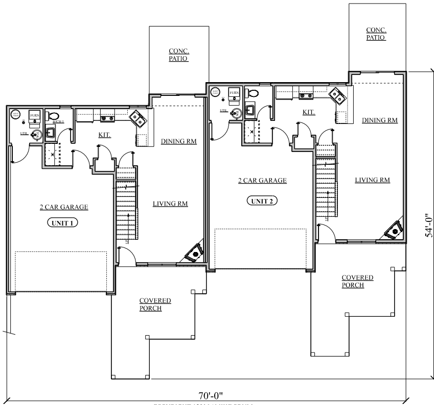
COPYRIGHT / 2016 / MIKE PRULL MAIN FLOOR PLAN
