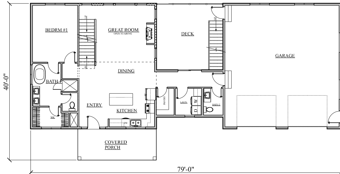
COPYRIGHT / 2024 / MIKE PRULL MAIN FLOOR PLAN
