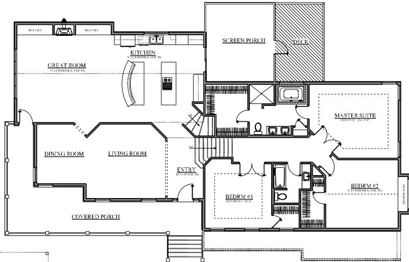
MAIN & UPPER FLOOR PLAN
