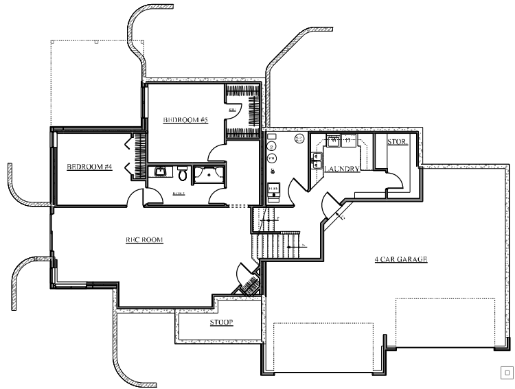
BASEMENT & LOWER FLOOR PLAN
