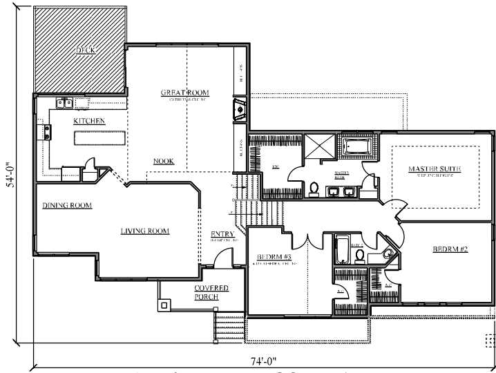
MAIN & UPPER FLOOR PLAN
