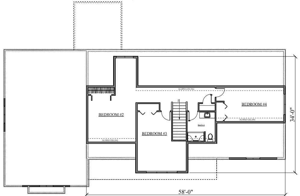
2ND FLOOR
