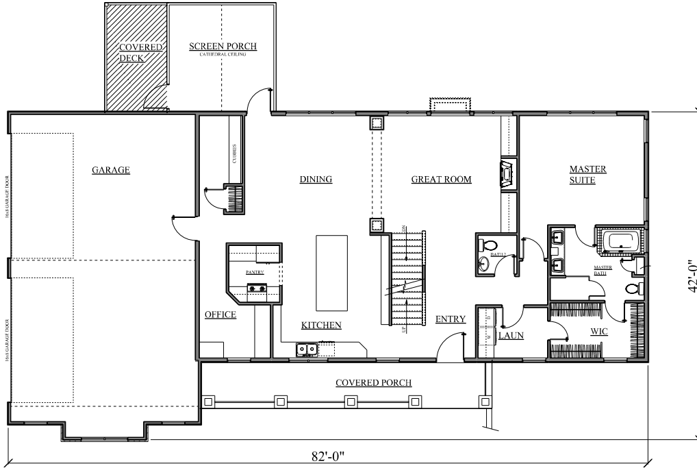
MAIN FLOOR
